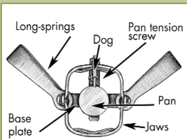
Figure BV9. Double jaw double-longspring trap (open)
