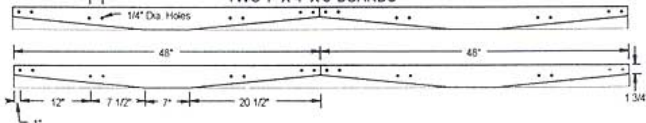
GOURD HANGERS TWO 1" X 4" X 8' BOARDS
