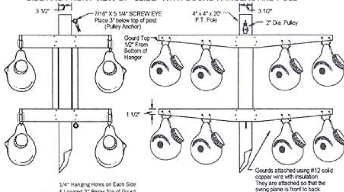
SIDE AND FRONT VIEW OF "SLIDE" WITH GOURD HANGERS AND POLE
